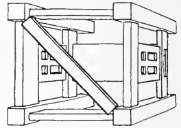
FIG. 421-b. ADJUSTING DIAGONALS.
